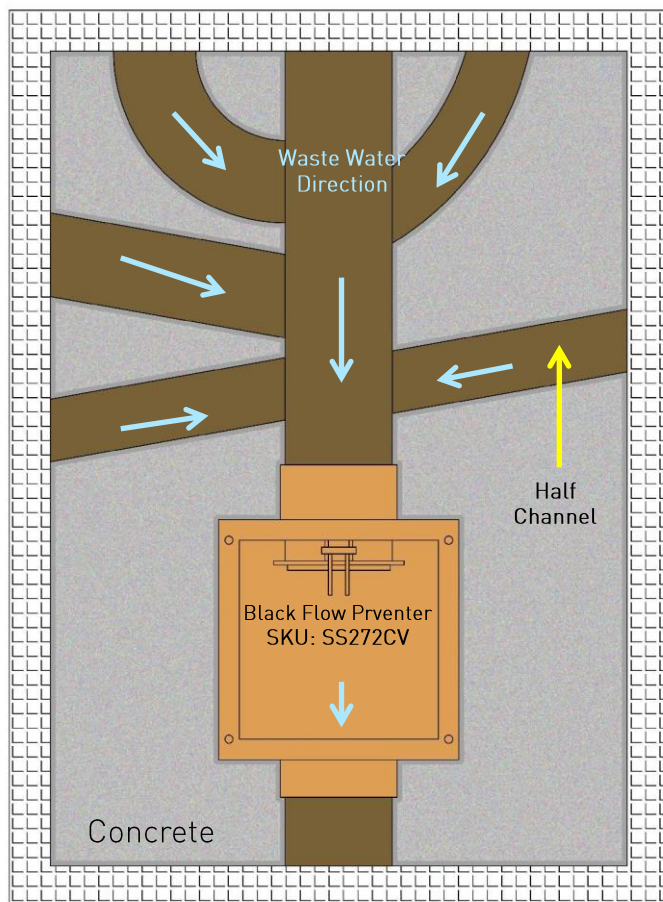
INSTALLATION ASSEMBLY
