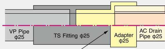
TS socket with the same nominal diameter
