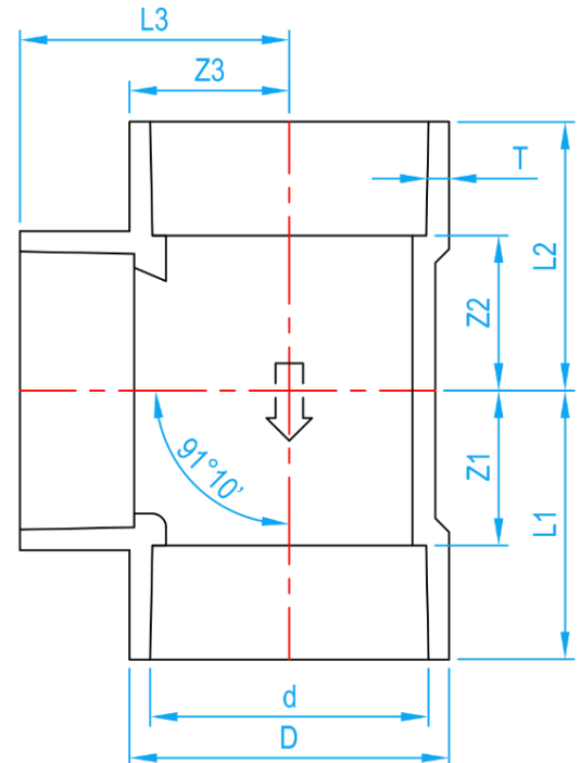
CROSS SECTIONAL VIEW
