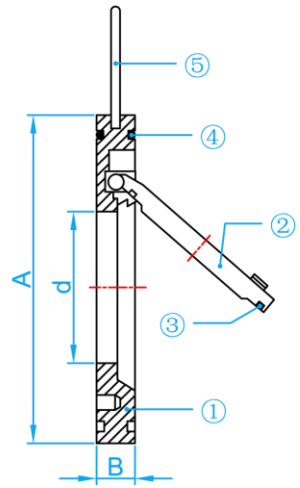
CROSS SECTIONAL VIEW
