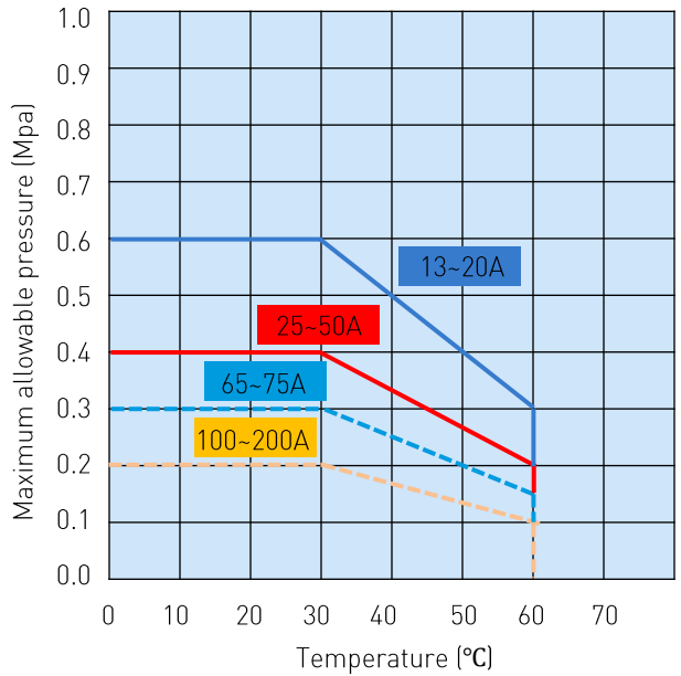
MAXIMUM ALLOWABLE PRESSURE AND TEMPERATURE
