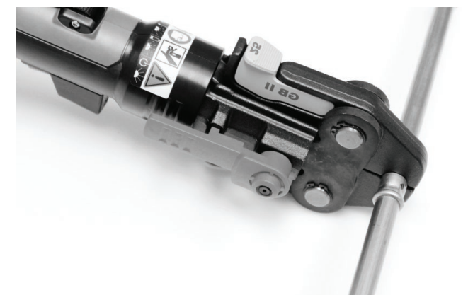
Figure 6 – Placing Scissor-Style Jaw Set Around Fitting
