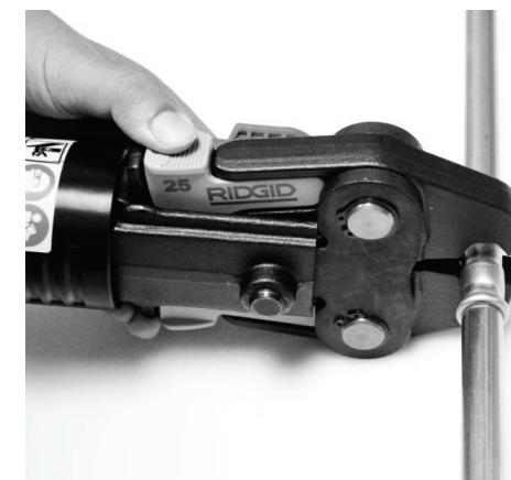
Figure 5 – Opening The Scissor-Style Jaws
