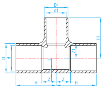
CROSS SECTIONAL VIEW
