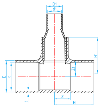
*WITH BUSHING CROSS SECTIONAL VIEW
