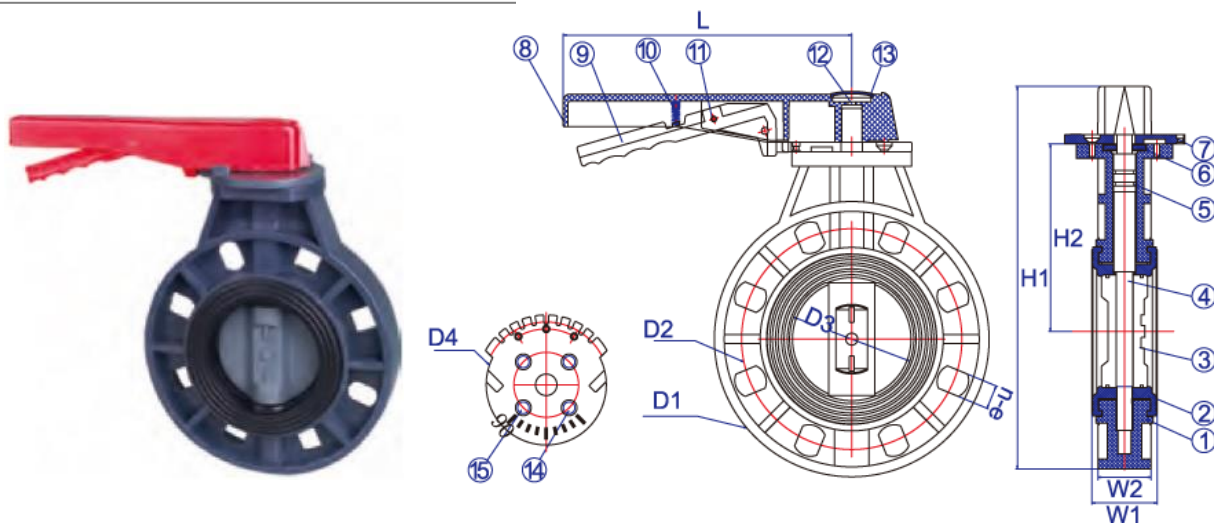
COMPONENT PARTS
